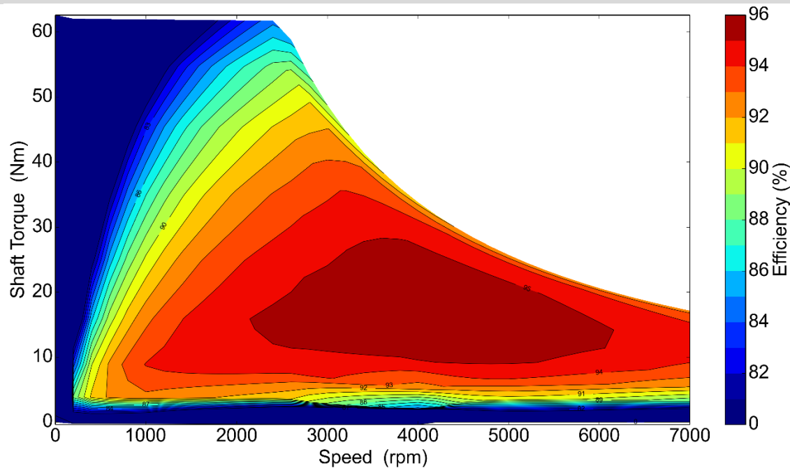
Efficiency Map % (*)
